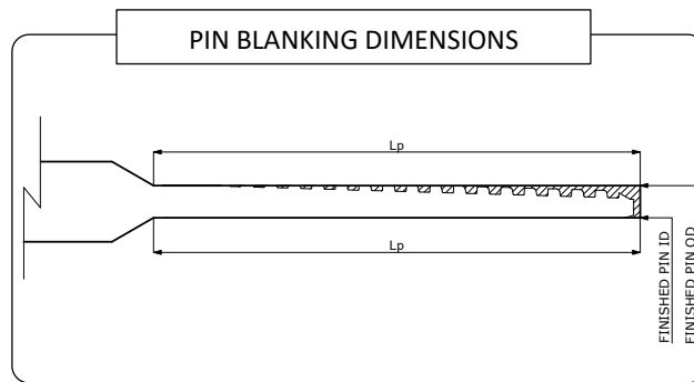
a) LENGTH OF L_p AND L_b DOES NOT INCLUDE RE-CUT LENGTH.
