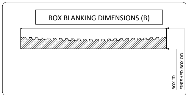
b) When Box OD is turned, aiming OD tolerance is +/- 0.015".
